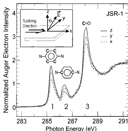
Figure 2. NEXAFS spectra recorded for sample JSR-1 with E \parallel x (dashed line), y (dotted line) and 20^\circ from the z axis (solid line). The experimental geometry is shown in the inset. The buffing direction is taken along the x axis. By rotation of the sample around the z axis, the E vector of the incident X-rays could be oriented in either the x - z plane or y - z plane. The polar angle \theta was changed by rotating the sample about an axis in the surface plane. The assignment of the observed peaks 1–3 to \pi^* orbitals of chemically different C atoms is also indicated.
